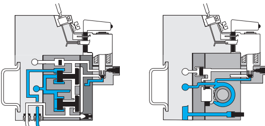
Modul 4/2 monostabil
