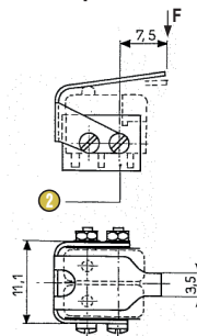
2 3 insulating plates
