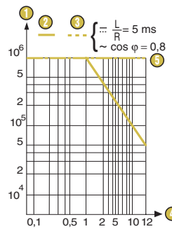
Operating curve for type 83264
