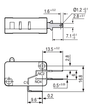
X3 for printed circuit board, front output
