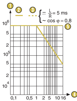
Operating curve for types 83261 / 83263
