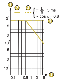
Operating curve for type 83265
