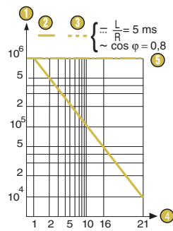
Operating curve for type 83262
