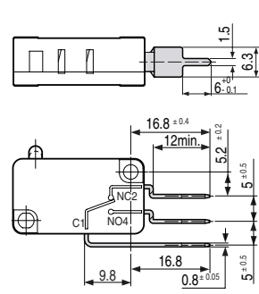
W3R2.5 for RAST 2.5 connector (SP9307)
