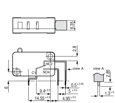
W3R2.5 for RAST 2.5 connector (SP9307)
